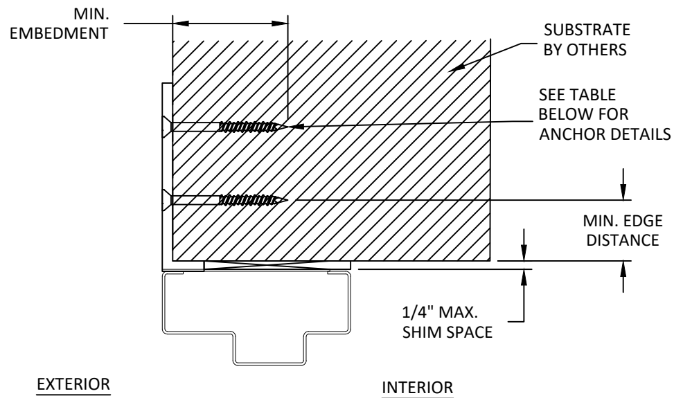
A 6 VERTICAL SECTION HEAD - STRAP NOTE: JAMB SIMILAR
