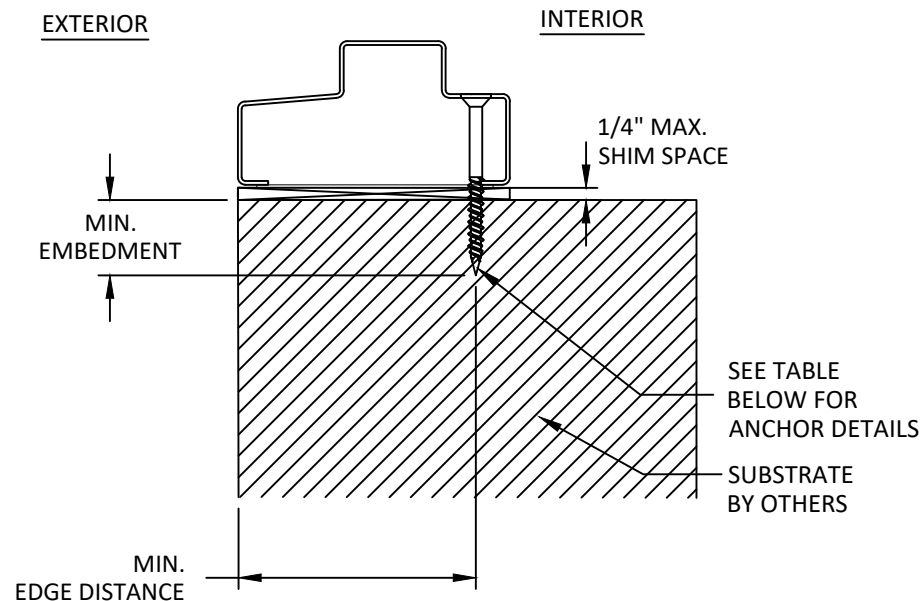
B 6 VERTICAL SECTION SILL - THROUGH FRAME
